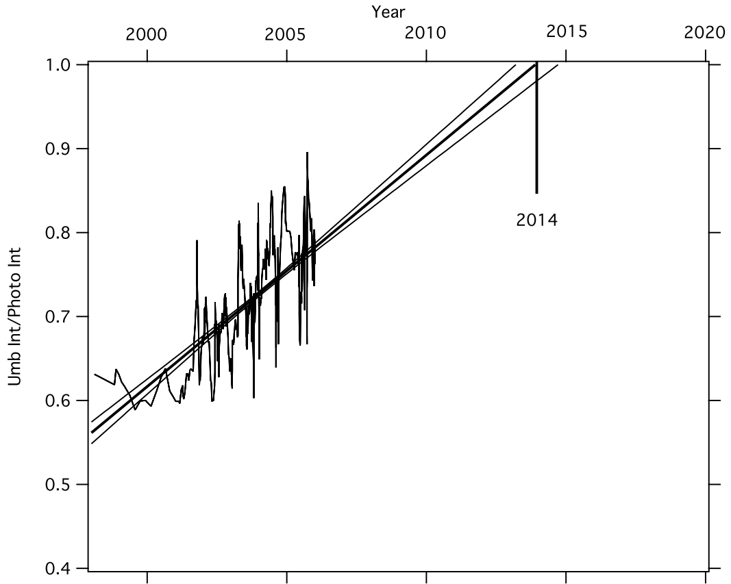
Figure 4 – A linear fit to the observed umbral contrast values, extrapolated to show that by 2014 the average umbrae would have the same brightness as the quiet Sun.
